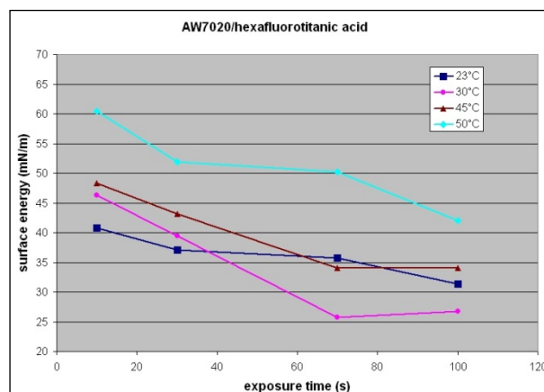
Fig.1b: SFE of AW7020 as a function of the conversion bath exposure time
